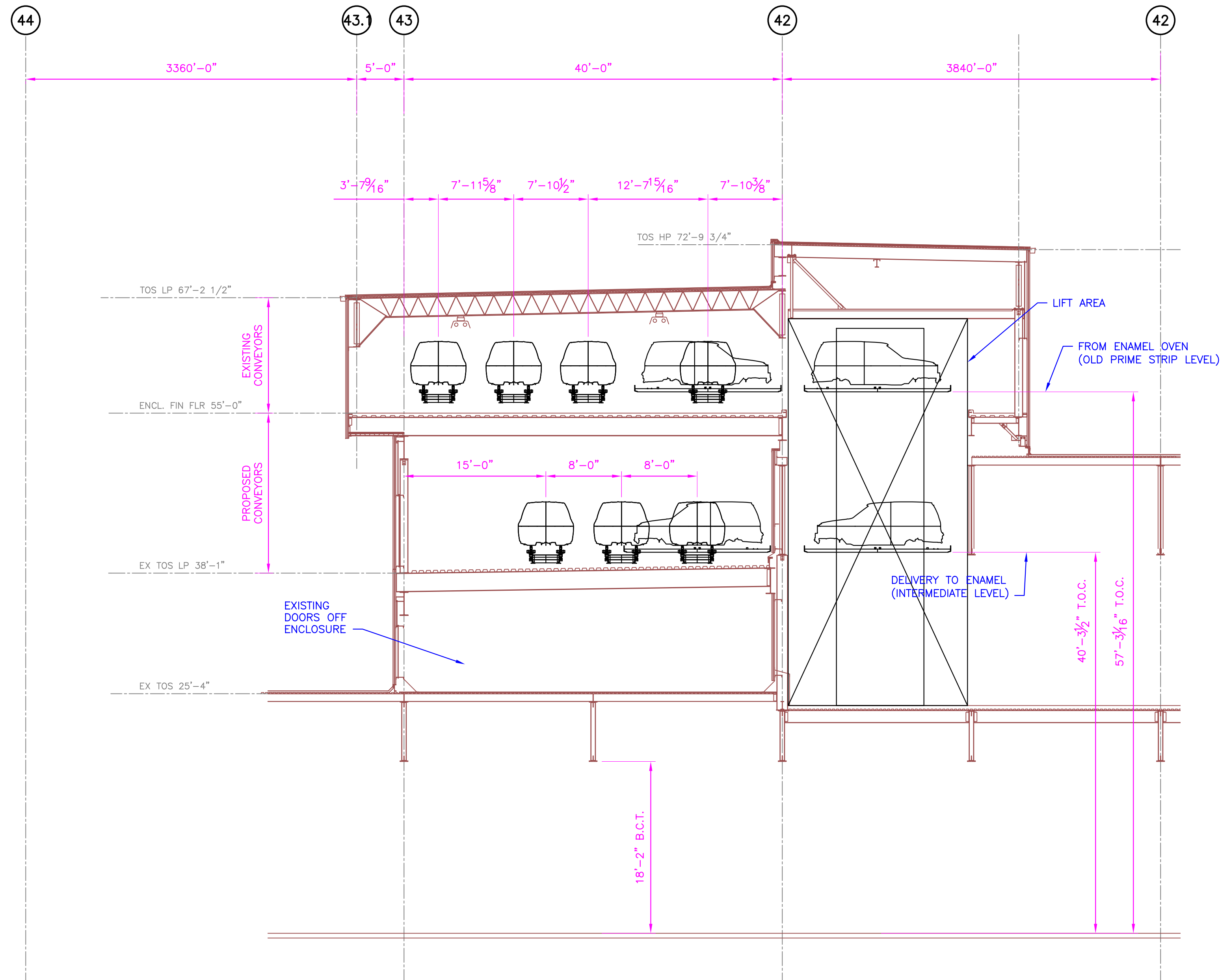
C OA1 KANSAS CITY SUV ENAMEL DELIVERY/LIFTS CROSS SECTION SCALE: 1/8" = 1'-0"
