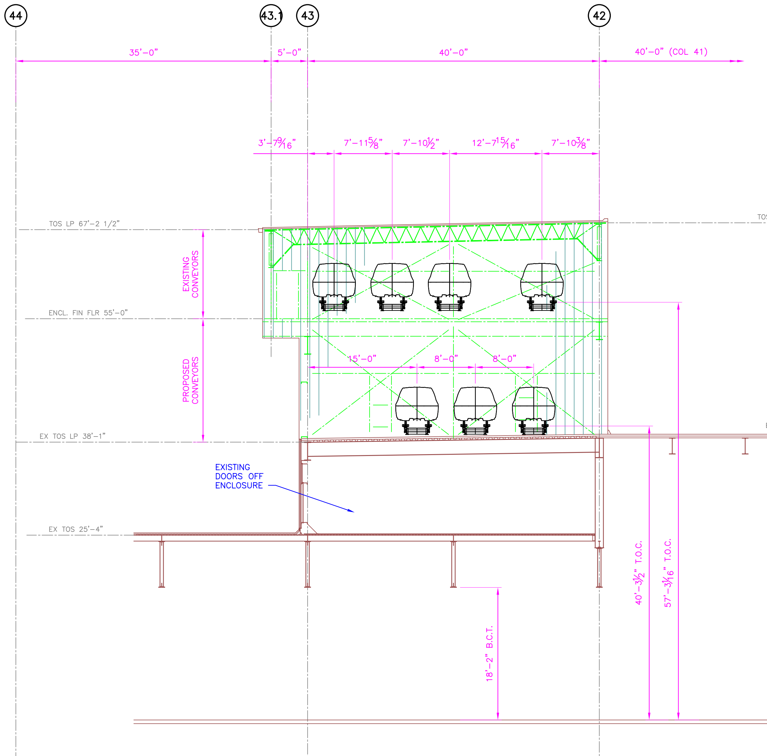
B OA1 KANSAS CITY SUV ENAMEL DELIVERY CROSS SECTION SCALE: 1/8" = 1'-0"
