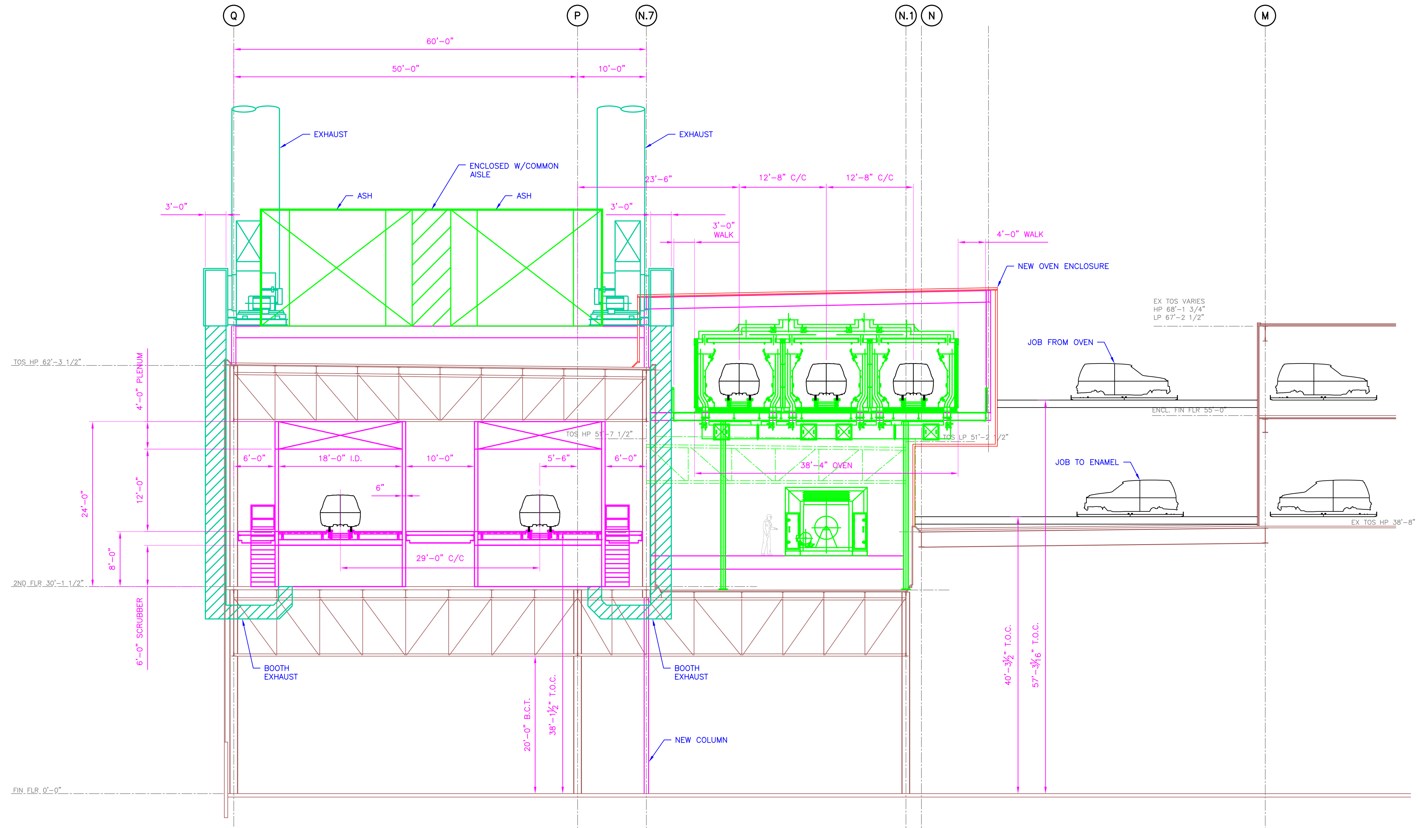
A OA1 KANSAS CITY SUV ENAMEL BOOTH & OVEN CROSS SECTION SCALE: 1/8" = 1'-0"
