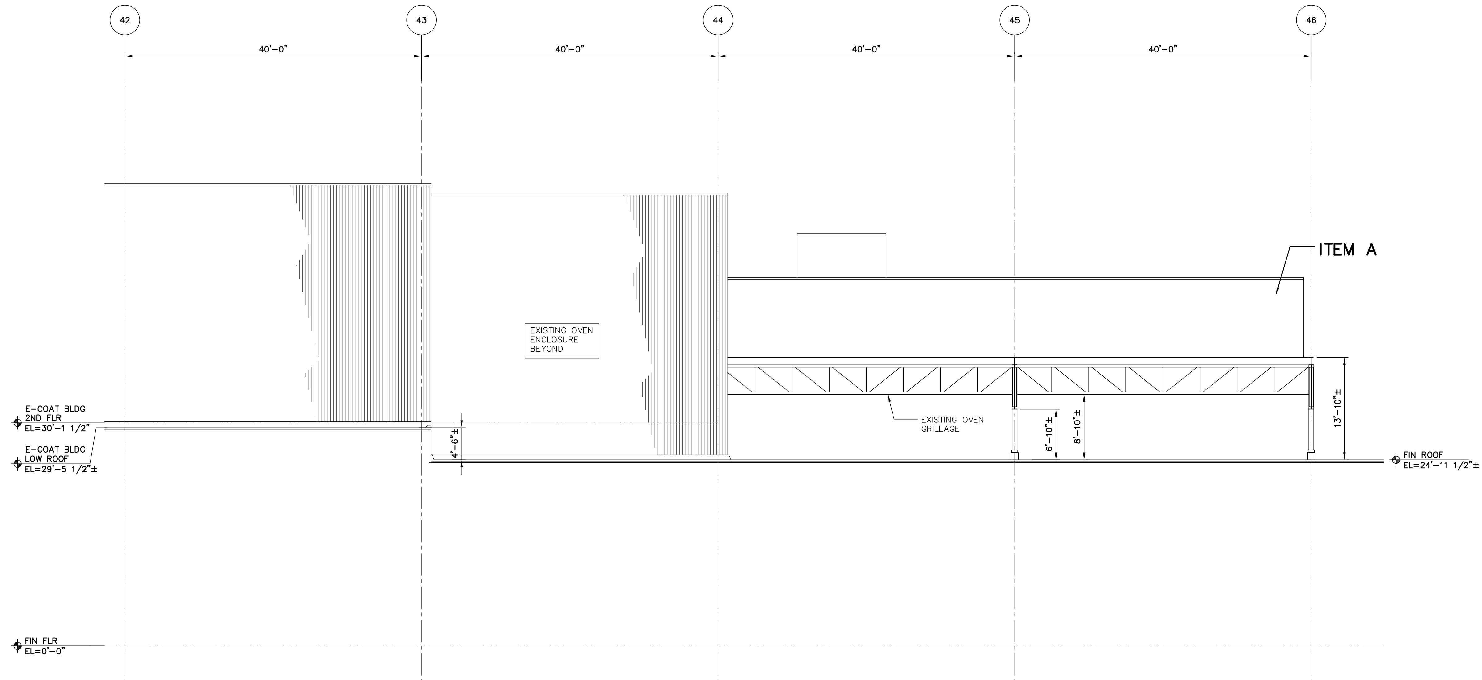
4 BUILDING SECTION (EXISTING CONDITION) A-1 SCALE: 1/8" = 1'-0"
