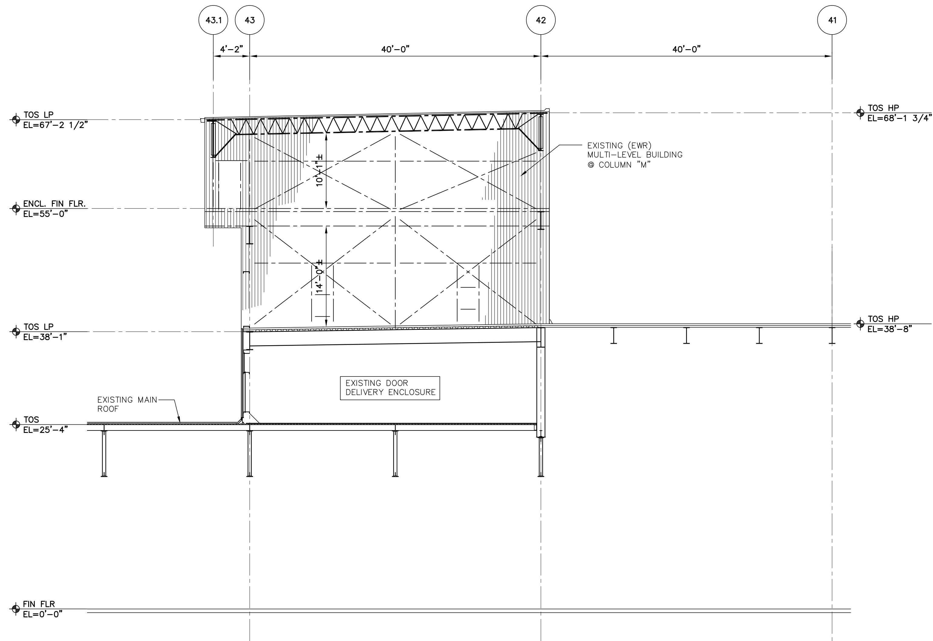
2 BUILDING SECTION/ELEVATION A-1 SCALE: 1/8" = 1'-0"
